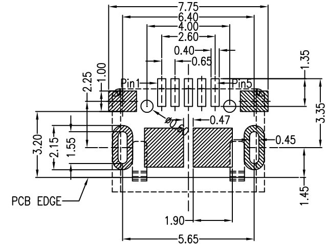
RECOMMENDED PCB LAYOUT PCB图仅供参考
