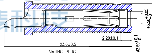
MATING PLUG
