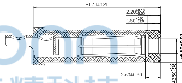
MATING PLUG
