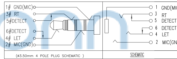
(ø3.50mm 4 POLE PLUG SCHEMATIC )
