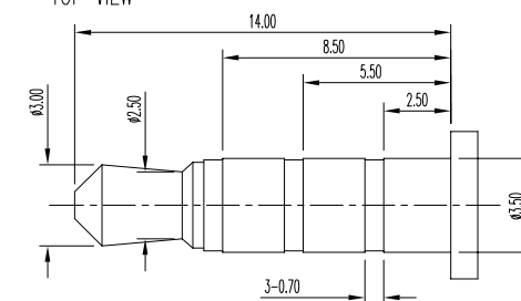
(ø3.50mm 4 POLE PLUG DETAIL DRAWING)
