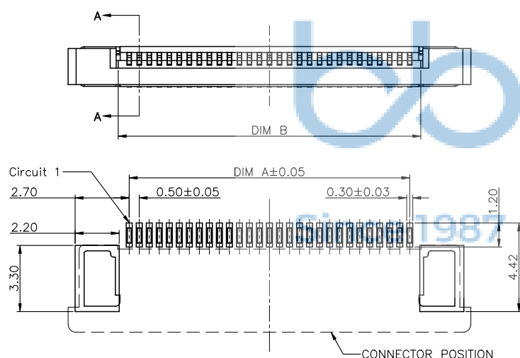
RECOMMENDED P.C.B PATTERN LAYOUT
