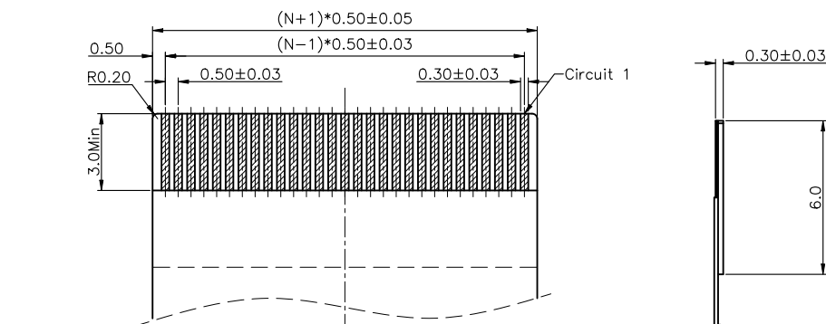
RECOMMENDED FPC/FFC DIMENSION
