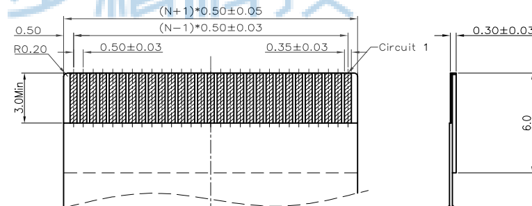
RECOMMENDED FPC/FFC DIMENSION
