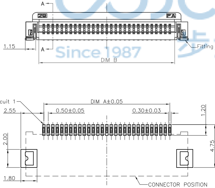
RECOMMENDED P.C.B PATTERN LAYOUT
