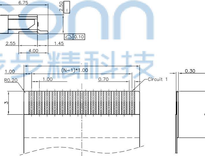
RECOMMENDED FPC/FFC DIMENSION
