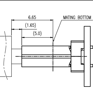
MATED CONDITION (REF)
