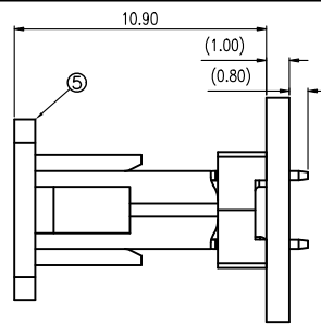
CAP ASSEMBLY AND MOUNTING CONDITION (REF)
