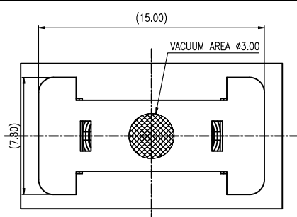
CAP ASSEMBLY AND MOUNTING CONDITION (REF)
