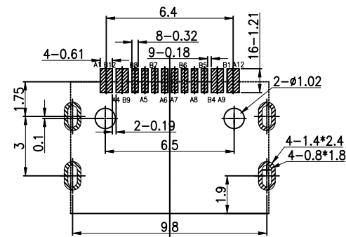
RECOMMENDED PCB LAYOUT Tolerance: \pm 0.05\text{mm}
