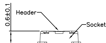
Matting drawing
