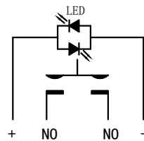
Principle diagram of monochrome electrical apparatus
