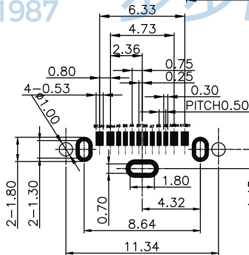
RECOMMENDED PCB LAYOUT(TOP VIEW) (GENERAL TOLERANCE±0.05)
