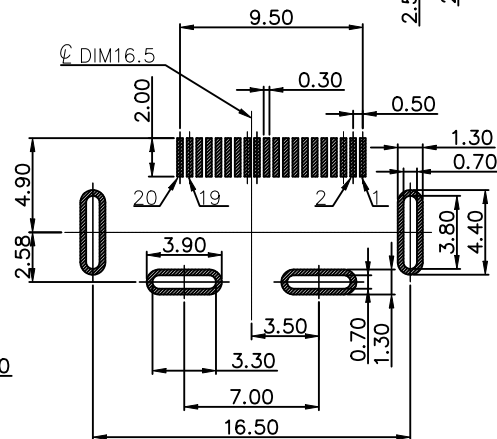
RECOMMEND P.C.B. LAYOUT(TOP VIEW) (P.C.B THICKNESS=1.60mm)
