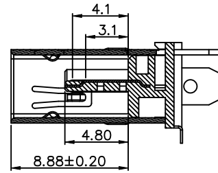
SEC.A-A VIEW ROTATE 90°
