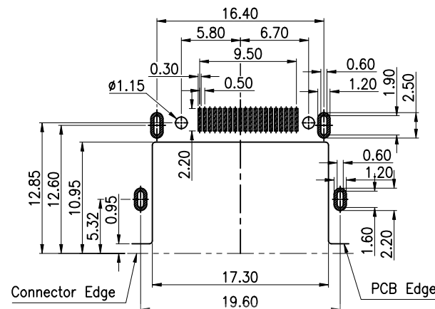
RECOMMENDED PCB LAYOUT (THICKNESS=1.60±0.05mm)
