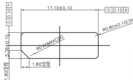
REFERENCE PANEL CUT OUT DIMENSIONS
