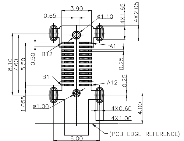
RECOMMENDED P.C.B LAYOUT TOLERANCE ± 0.05mm (TOP VIEW)
