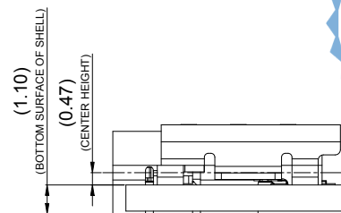
MOUTING CONDITION(REF.)
