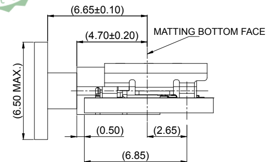
MATED CONDITION(REF.)
