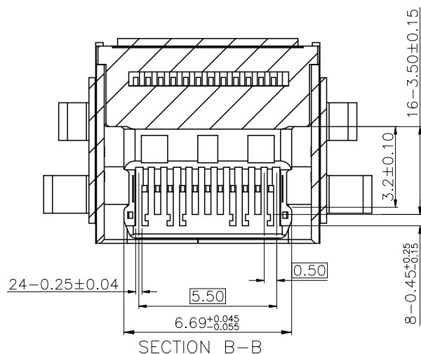
SECTION B-B
