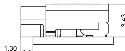
MOUNTING CONDITION(REF.)
