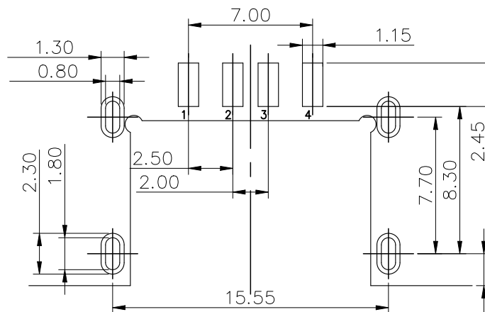
RECOMMENDED P.C.B HOLE LAYOUT COMPONENT SIDE VIEW (TOLERANCE: \pm 0.05 )
