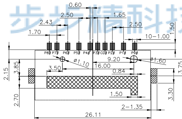
PCB LAYOUT TOP VIEW (TOLERANCE: \pm 0.05 )
