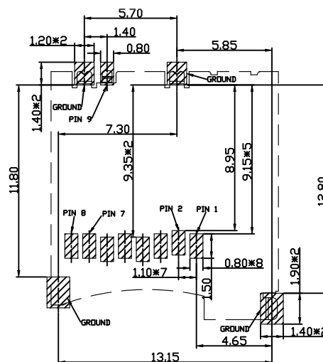
RECOMMENDED PCB LAYOUT (ALL TOLERANCE ARE ±0.05)
