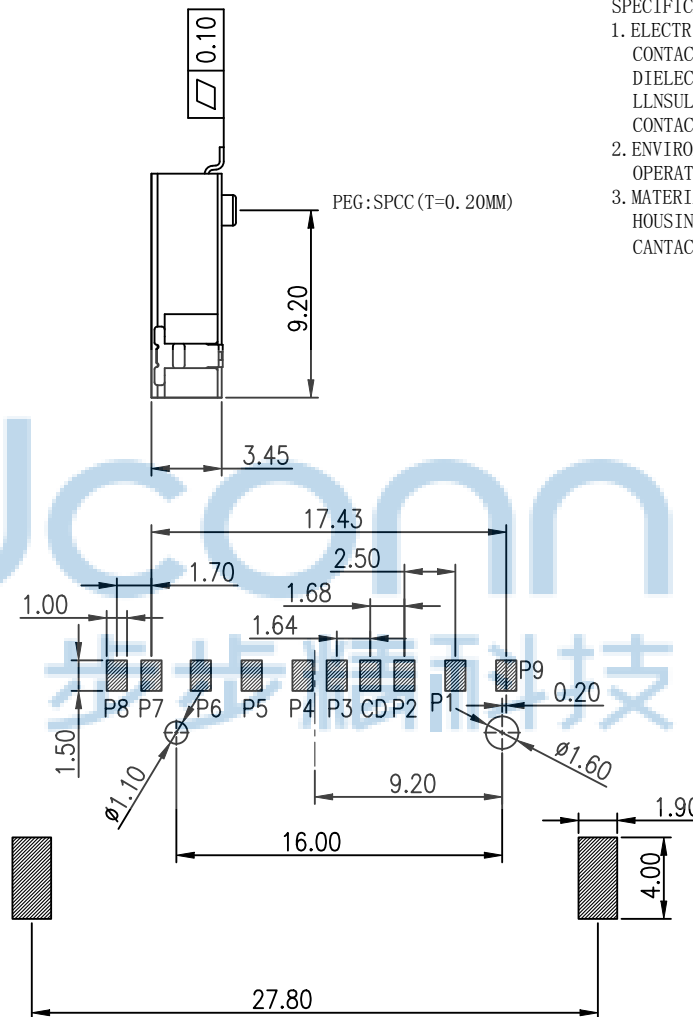
PCB LAYOUT TOP VIEW (TOLERANCE:±0.05)
