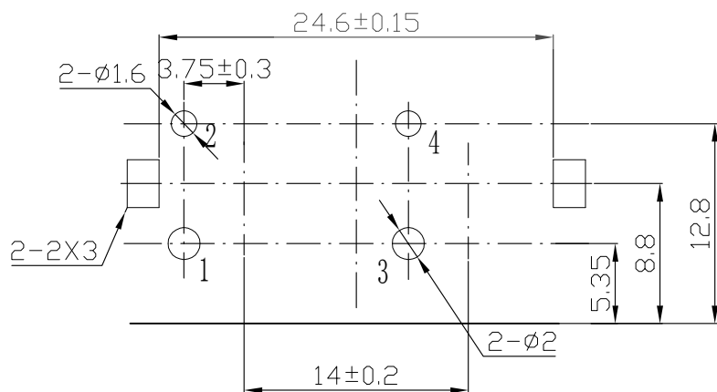
P. C. B LAYOUT (TOP VIEW) Tolerance: \pm 0.05
