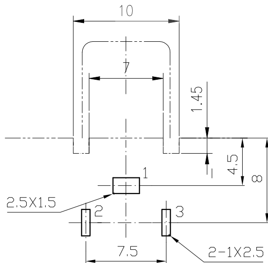
PCB LAYOUT(TOP VIEW) Tolerance:±0.05
