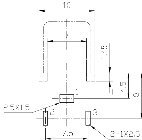
PCB LAYOUT(TOP VIEW) Tolerance:±0.05
