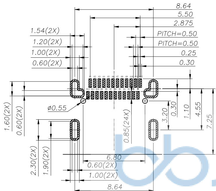
RECOMMENDED PCB LAYOUT(TOP VIEW) THICKNESS 1.60MM;DEFAULT TOLERANCE:±0.05
