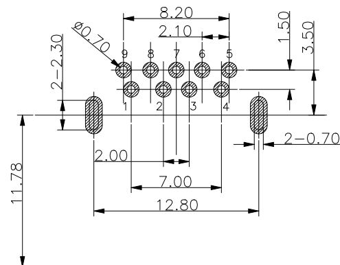
RECOMMENDED PCBA LAYOUT (TOLERANCE+/-0.05)
