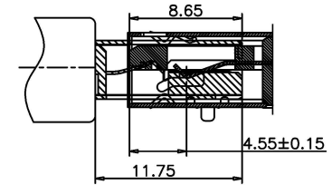
Receptacle and plug mating drawing
