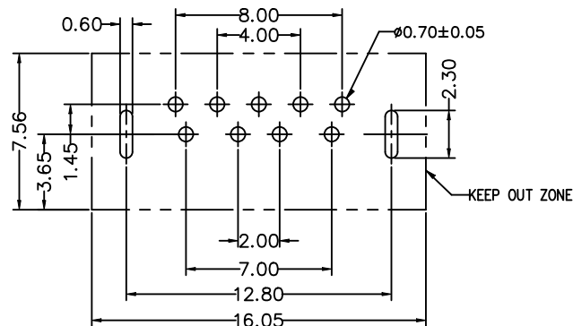
Recommended PCB Layout PCB Thickness=1.8±0.1mm
