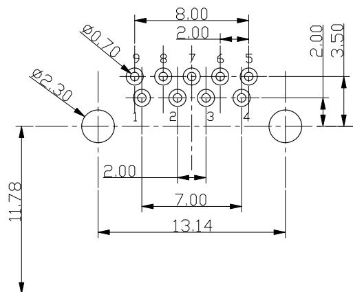
RECOMMENDED PCBA LAYOUT (TOLERANCE+ \pm 0.05 )
