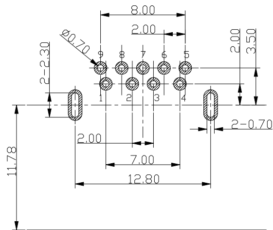
RECOMMENDED PCBA LAYOUT (TOLERANCE+ \pm 0.05 )
