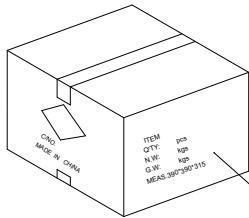
BOX DIMENSIONS: 390*390*315
