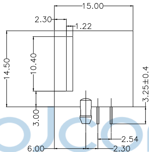
CUTAWAY VIEW
