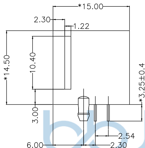
CUTAWAY VIEW
