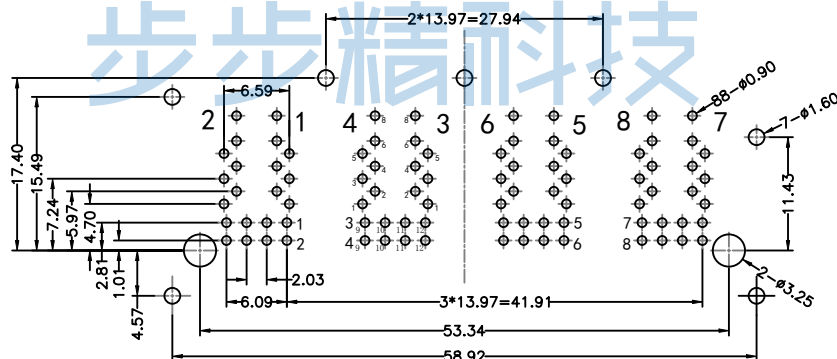
RECOMMENDED PCB LAYOUT VIEWED FROM COMPONENT SIDE
