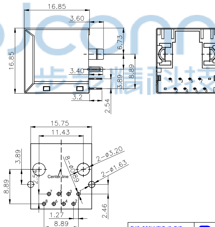
RECOMMENDED PCB LAYOUT VIEWED FROM COMPONENT SIDE
