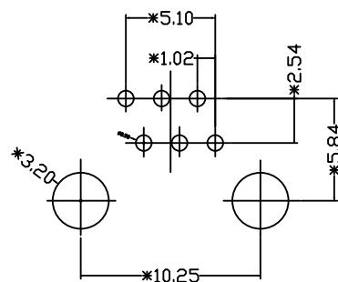
PCB LAYOUT THICKNESS=1.6mm
