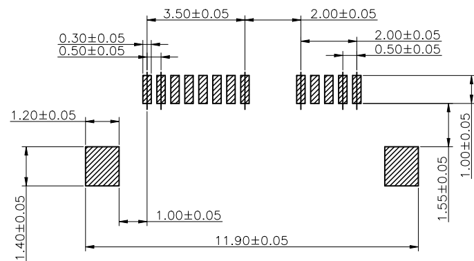
RECOMMENDED P.C.B PATTERN LAYOUT (TOP VIEW)
