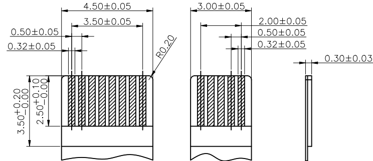
RECOMMENDED FPC/FFC DIMENSION (TOP VIEW)
