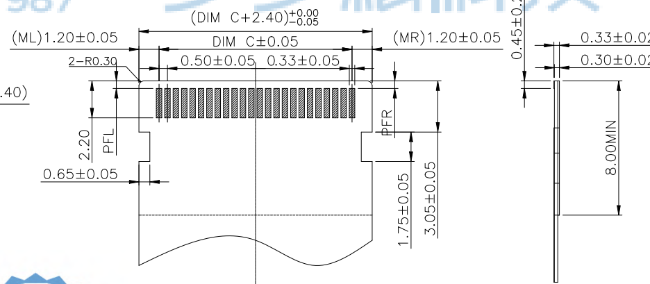
RECOMMENDED FPC/FFC DIMENSION
