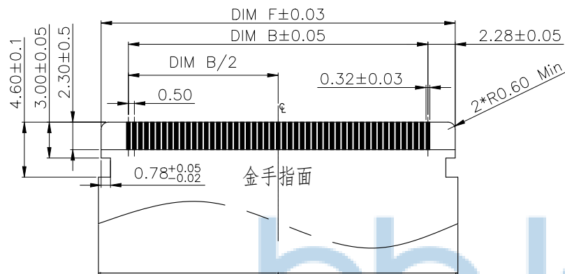
APPLICABLE FPC RECOMMENDED DIMENSION 一体覆膜FPC线
