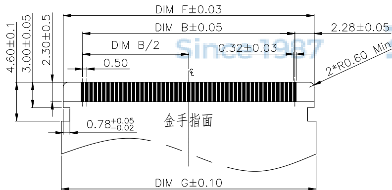
APPLICABLE FPC RECOMMENDED DIMENSION 一体覆膜FPC线
