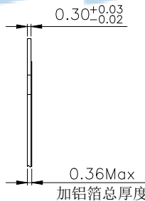
APPLICABLE FPC RECOMMENDED DIMENSION 贴铝箔FPC线
