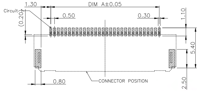
RECOMMENDED P.C.B PATTERN LAYOUT GENERAL TOLERANCE ±0.05
