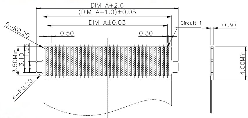
RECOMMENDED FPC/FFC DIMENSION GENERAL TOLERANCE ±0.05
