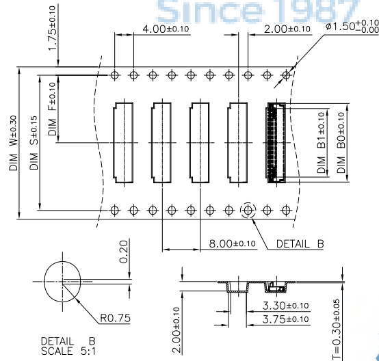
49~61PIN REEL
