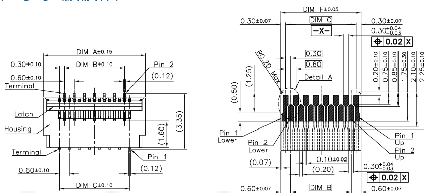
RECOMMENDED FPC
