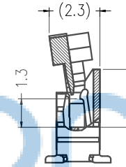
SECTION A-A Without cover
