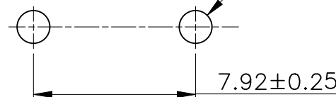
SUGGESTED PCB LAYOUT (COMPONENT SIDE)
