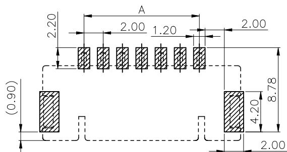
PCB LAYOUT(Tolerance:±0.05)
