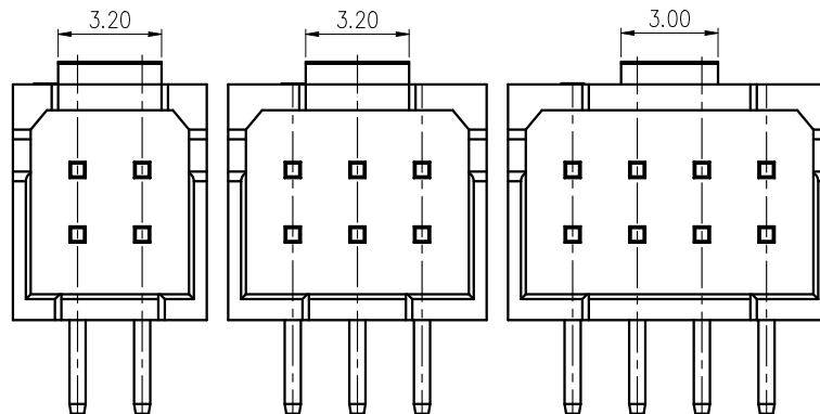
2~3P结构(2~3Pin Structure)
