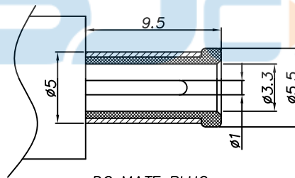
DC MATE PLUG
